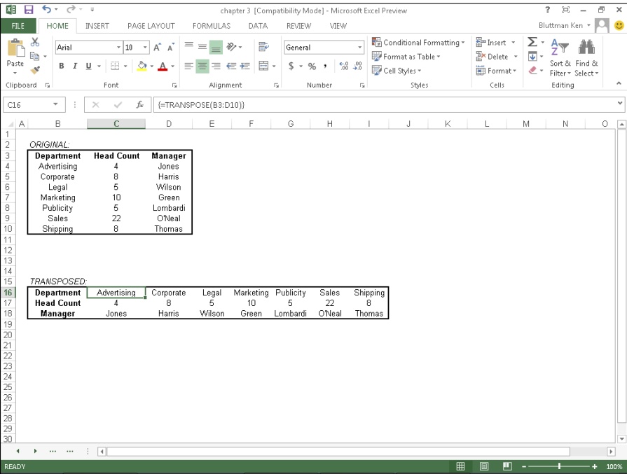
Figure 3-6: Transposing data.
